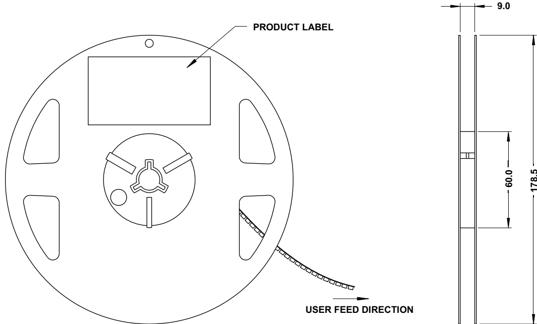
Figure 17: Reel Dimensions
