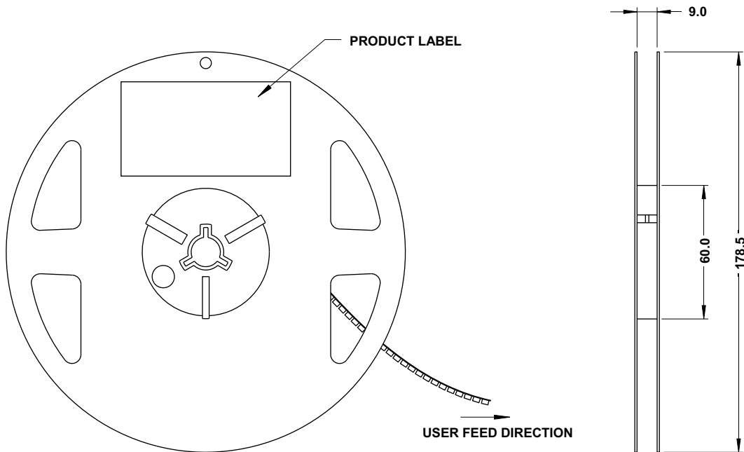
Figure 22: Reel Dimensions
