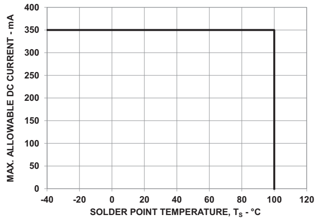
Figure 19: Maximum Forward Current vs. Solder Point Temperature. Derated based on T_{JMAX} = 125^{\circ}C , R_{\theta J-S} = 20^{\circ}C/W
