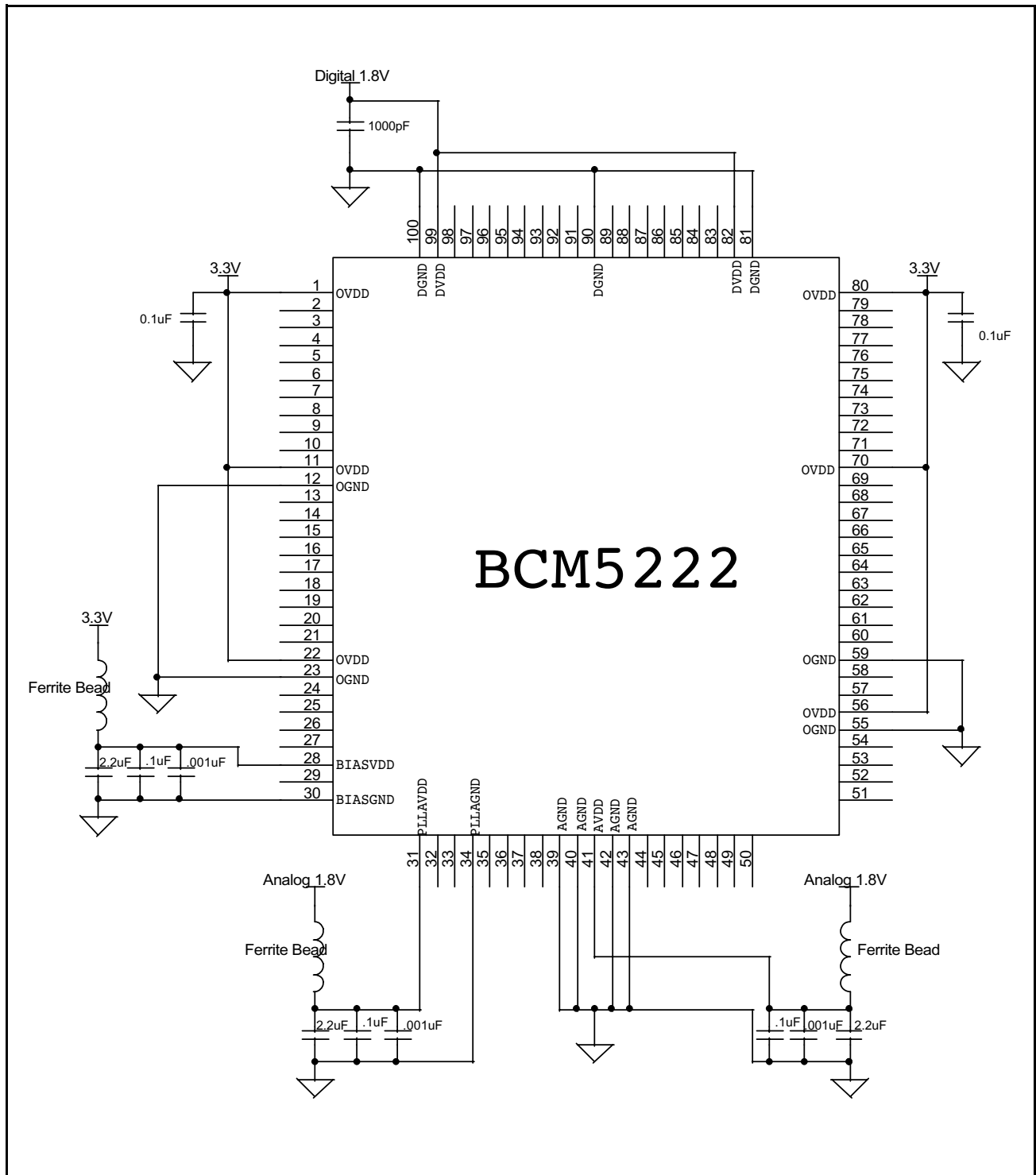
Figure 17: Power Connections BCM5222 (1.8V, 3.3V) (Shown in 100 MQFP package.)
