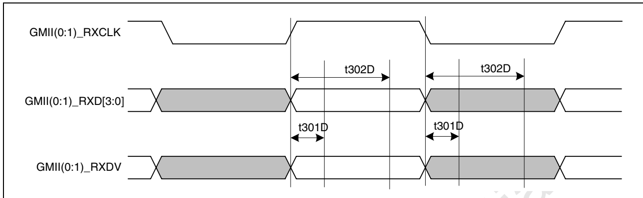
Figure 51: RGMI Input Timing (Delayed Mode Clock)
