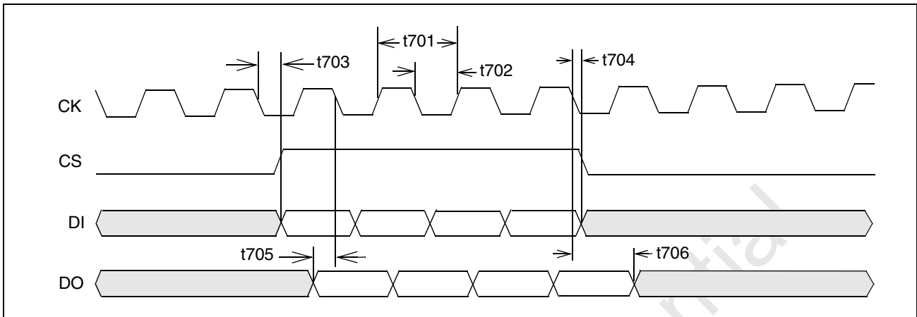
Figure 58: EEPROM Timing
