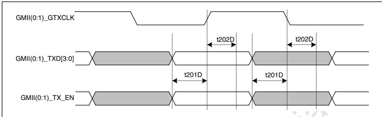
Figure 49: RGMI Output Timing (Delayed Mode Clock)
