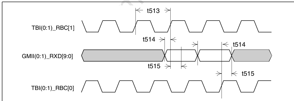
Figure 55: TBI Input Timing
