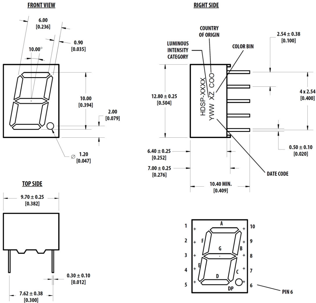
Figure 1: Package Drawing
