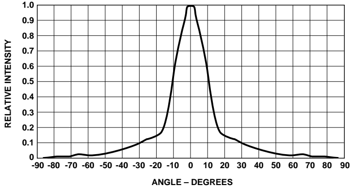
Figure 6. Relative luminous intensity vs. angular displacement for HLMP-Qxxx.
