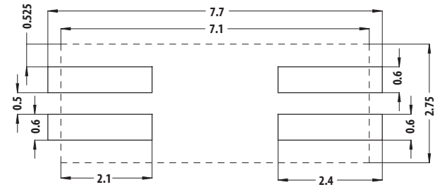
Figure 10. Land Pattern
