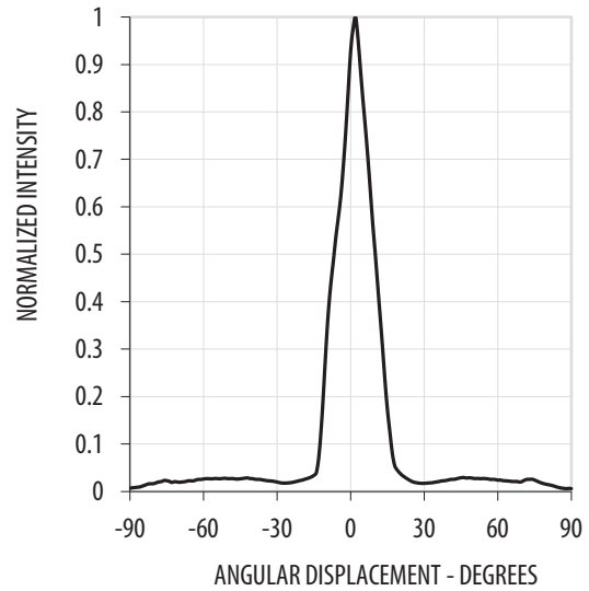
Figure 5: Radiation Pattern
