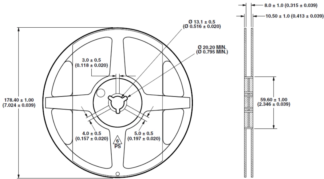
Figure 13: Reel Dimensions
