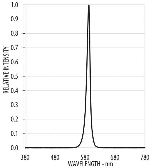
Figure 2: Spectrum
