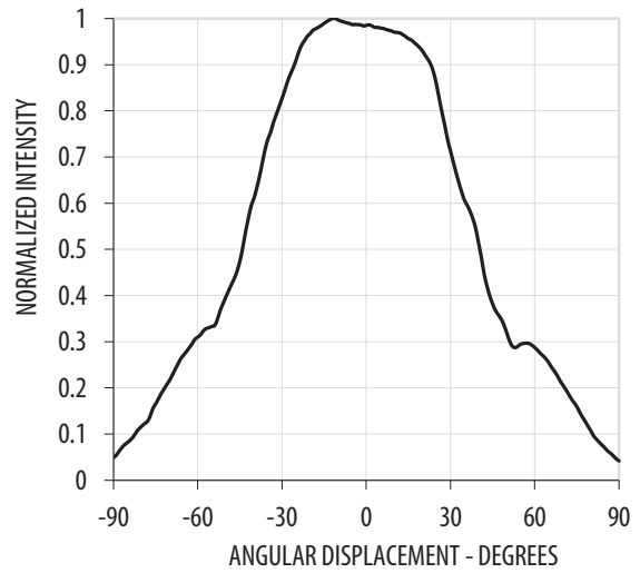
Figure 5: Radiation Pattern
