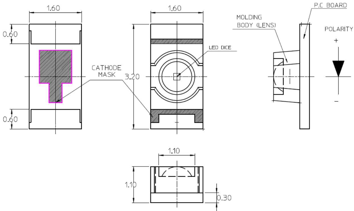
Figure 1: Package Dimensions
