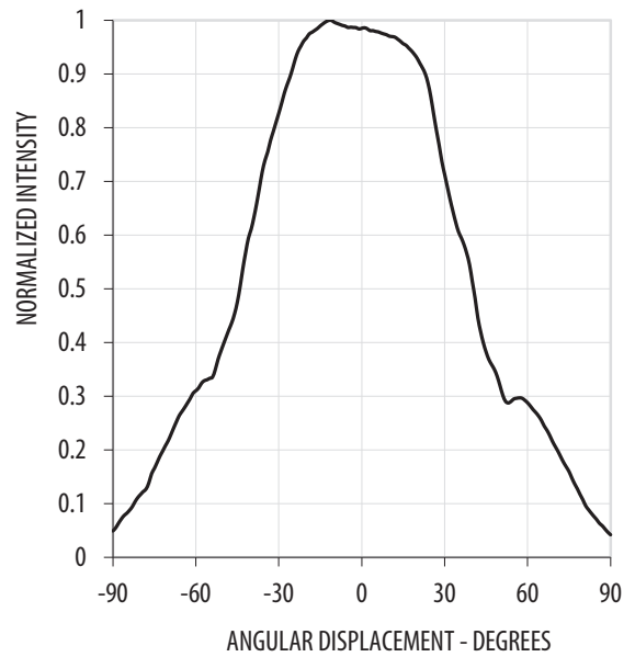
Figure 5: Radiation Pattern
