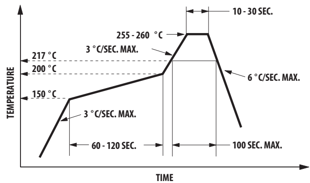
Figure 7. Recommended Pb-free reflow soldering profile. (Acc. to J-STD-020C)
