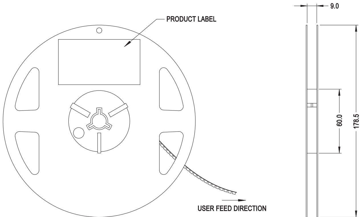
Figure 12: Reel Dimensions
