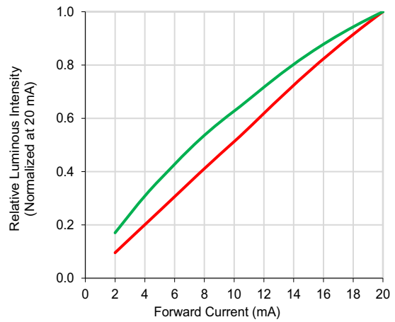
Figure 2: Relative Luminous Intensity vs. Forward Current
