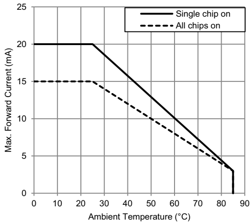
Figure 9: Derating Curve
