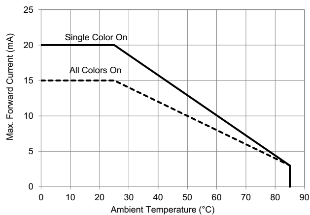
Figure 5: Derating Curve
