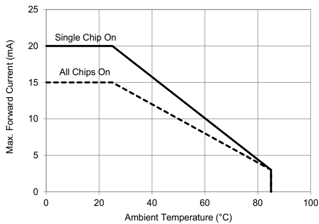
Figure 5: Derating Curve
