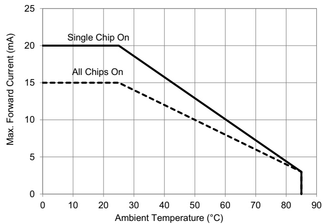
Figure 5: Derating Curve
