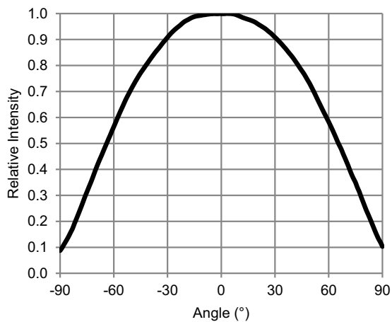
Figure 5: Relative Intensity vs. Angle
