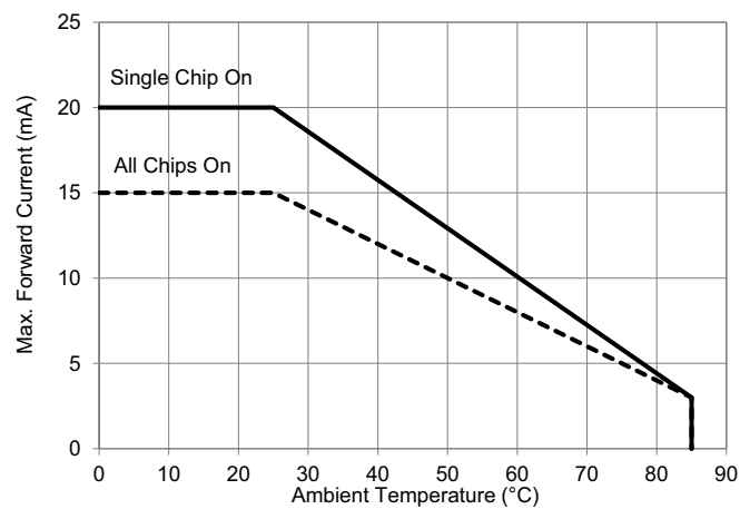
Figure 5: Derating Curve
