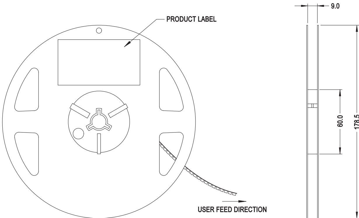
Figure 11: Reel Dimensions
