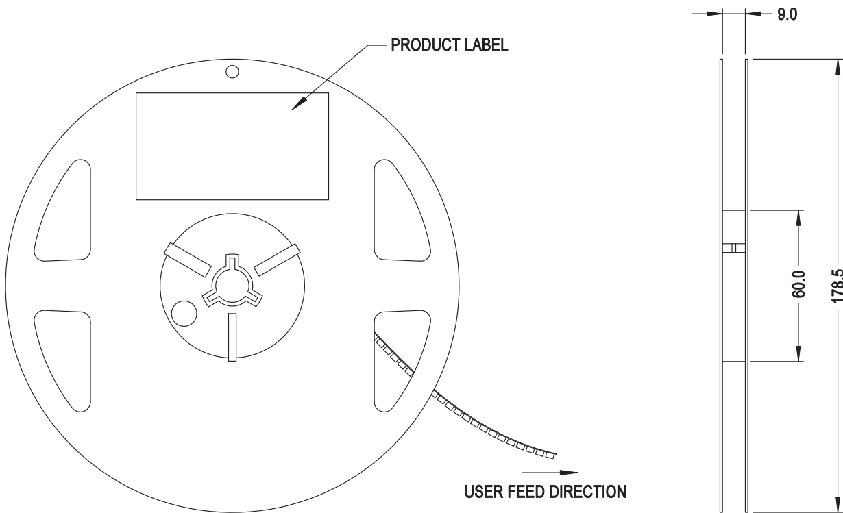
Figure 8: Reel Dimensions
