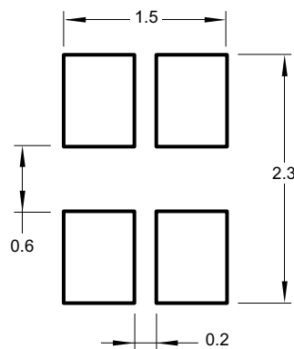
Figure 6: Recommended Soldering Land Pattern
