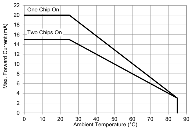
Figure 5: Derating Curve
