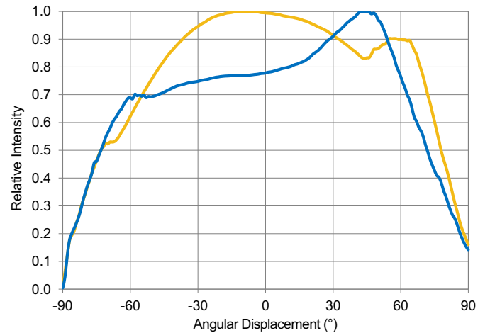
Figure 6: Radiation Pattern
