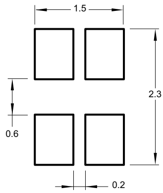
Figure 8: Recommended Soldering Land Pattern
