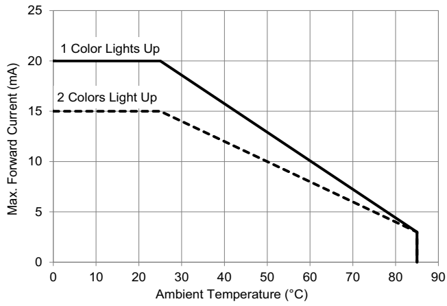
Figure 7: Derating Curve
