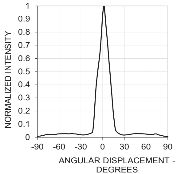
Figure 5: Radiation Pattern
