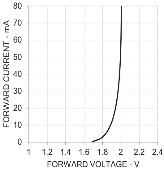
Figure 4: Forward Current vs. Forward Voltage
