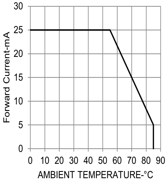
Figure 10: Derating Curve
