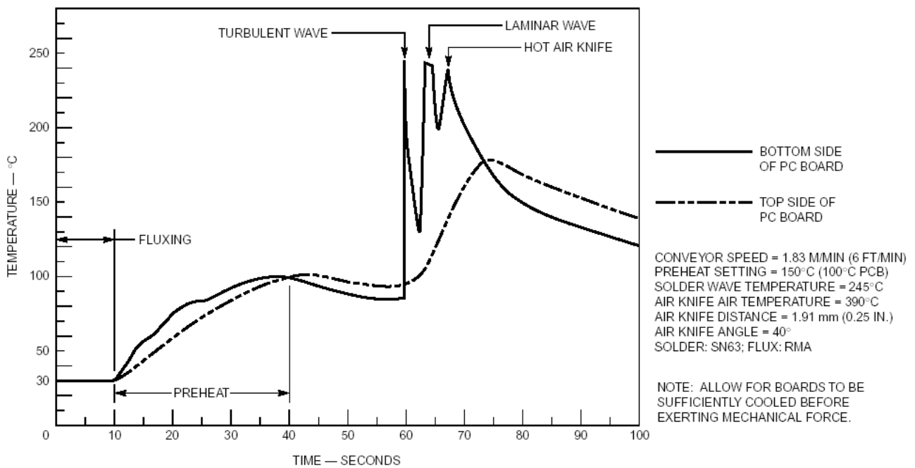
Figure 9. Recommended Wave Soldering Profile
