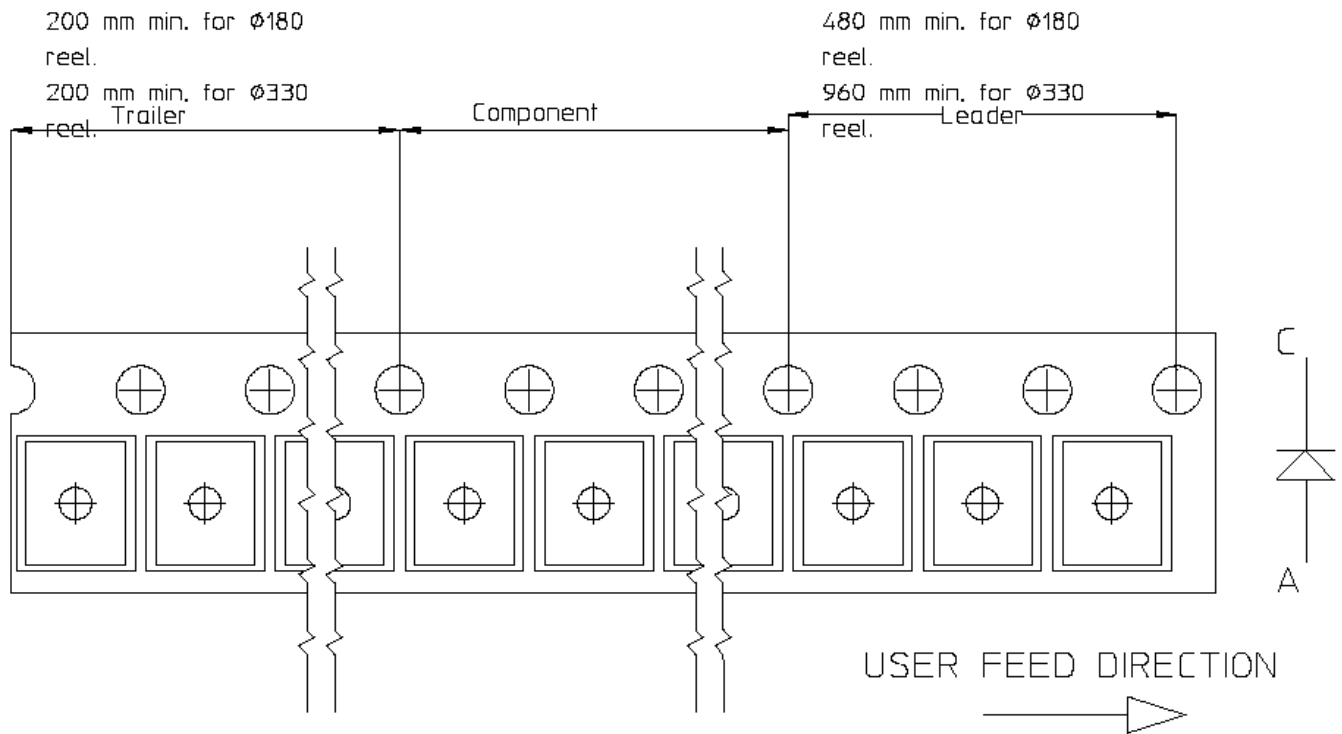
Figure 11. Tape leader and Trailer dimension
