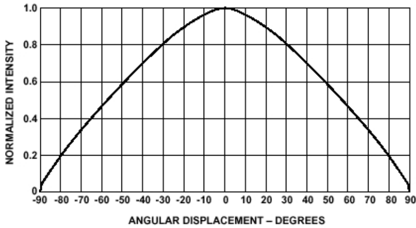
Figure 7. Radiation Pattern
