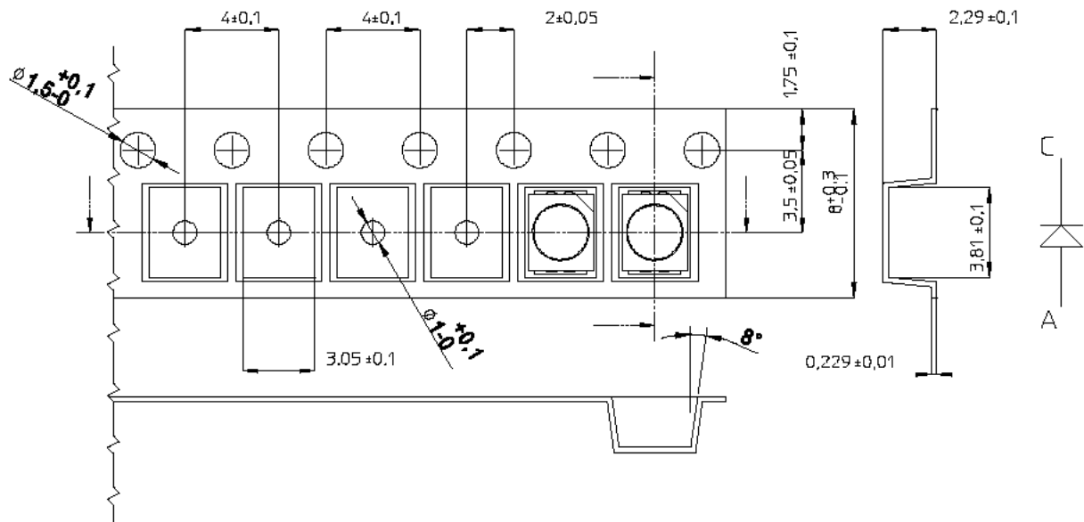
Figure 12. Tape dimension
