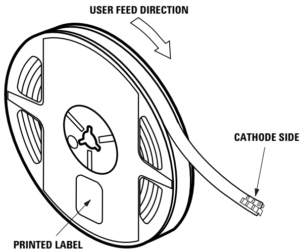
Figure 14. Reeling Orientation
