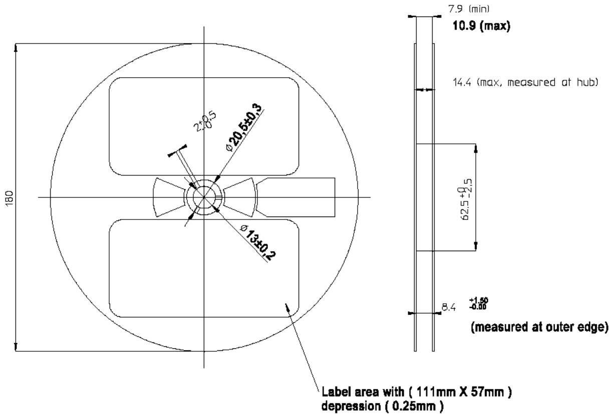
Figure 13. Reel dimension
