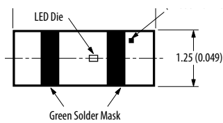
HSMx-C265
