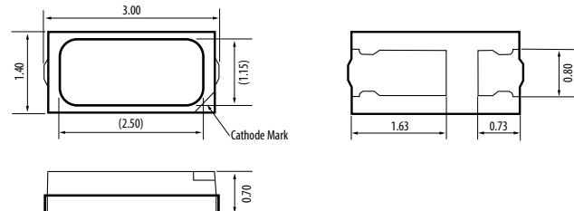
ASMD-LWG3/FWG3 -Nxxxx
