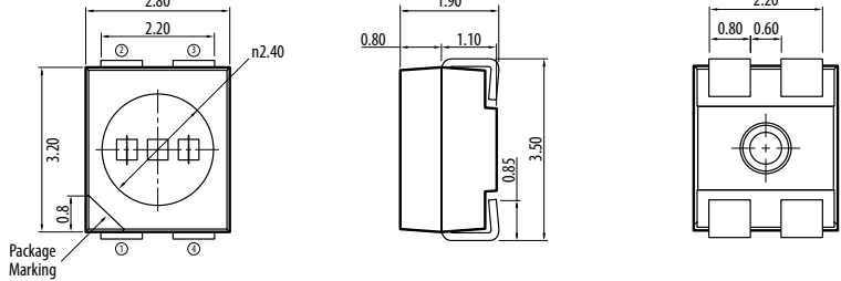
High Brightness Tricolor PLCC-4
