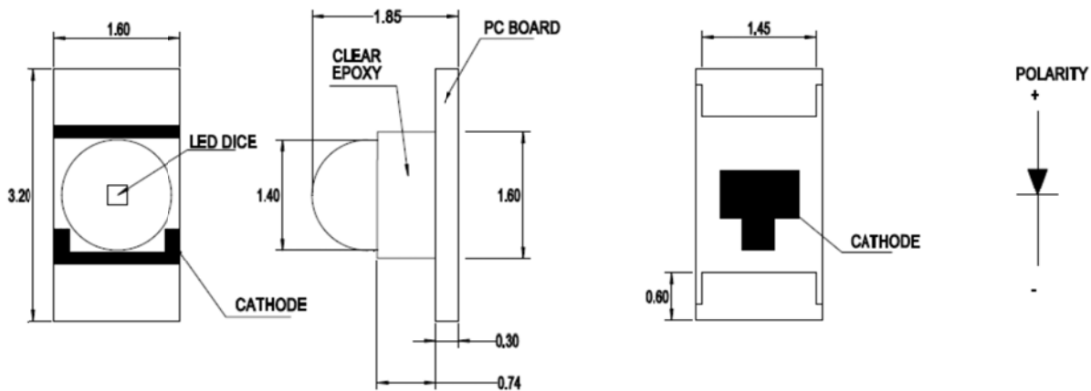
Figure 1: Package Dimensions
