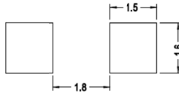
Figure 7: Recommended Soldering Land Pattern
