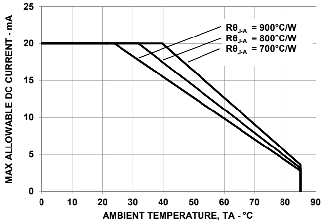
Figure 6: Derating Curve
