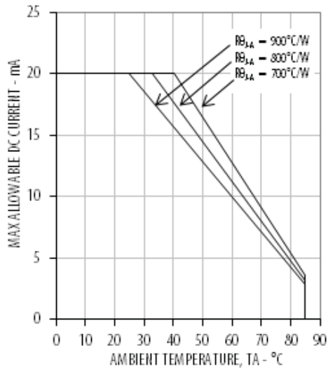
Figure 7 Derating Curve
