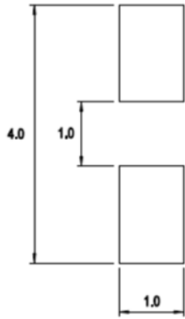
Figure 8: Recommended Soldering Land Pattern
