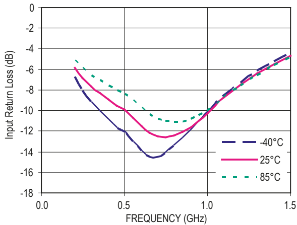
Figure 43. Input Return Loss vs Frequency ( V_d = 5V , I_{ds} = 15mA )
