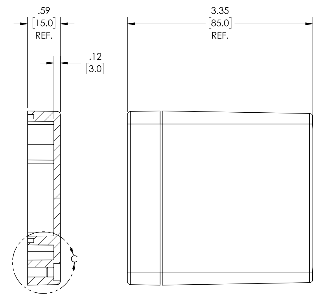
SECTION B-B
