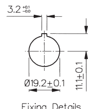
Fixing Details.
