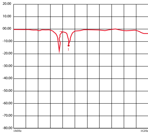
1 1450.00000 MHz -13.300 dB
