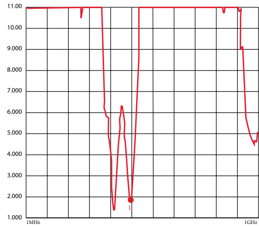
1 1450.00000 MHz -13.300 dB
