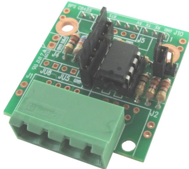
Removable 5.08mm Terminal Block Option
