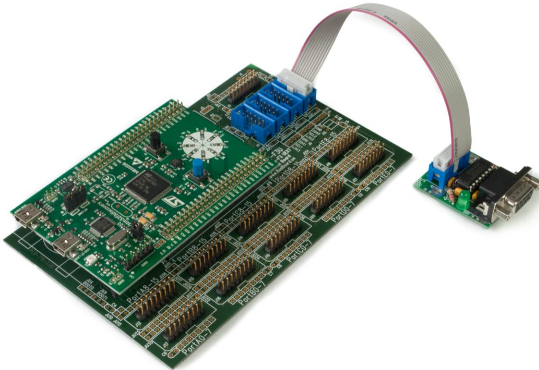
UEXT Module Attached to the STM32-F3U Discovery-F3 BaseBoard
