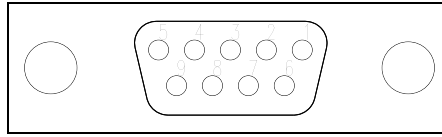
DB-9 Female Connector Pin Numbers For DCE Devices
