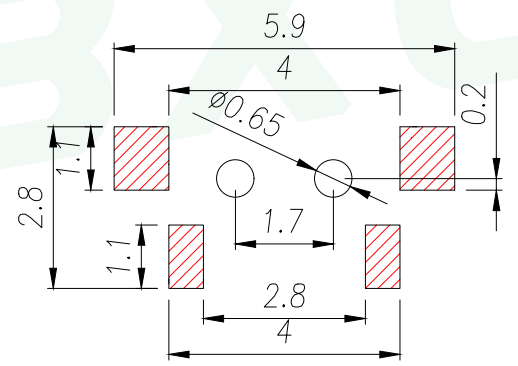
PCB.WELDING DRAWING
