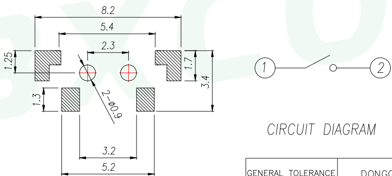
PCB.WELDING DRAWING
