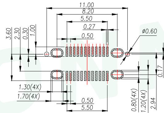
RECOMMENDED PCB LAYOUT(TOP VIEW) THICKNESS 1.0±0.10MM;DEFAULT TOLERANCE:±0.05
