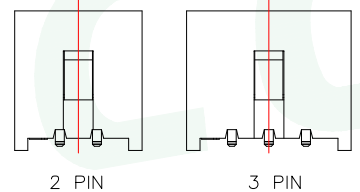
LOCK CONFIGURATION (脚位图)
