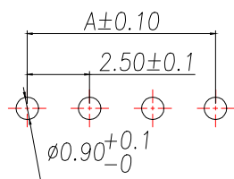
SUGGESTED PCB LAYOUT (COMPONENT SIDE)
