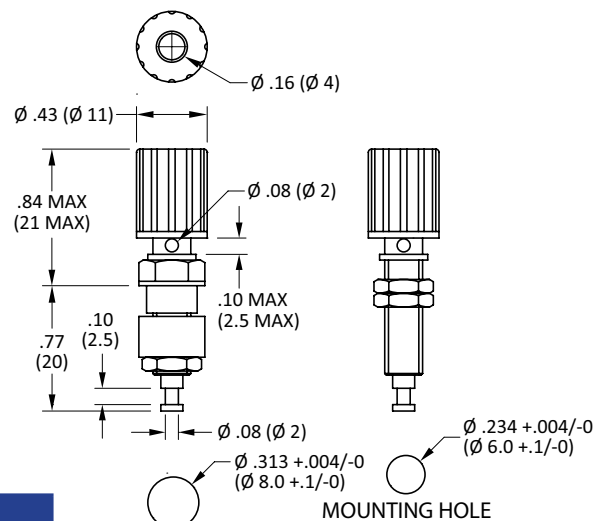
MOUNTING HOLE
