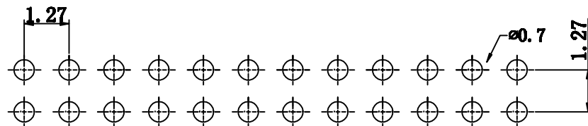
PCB LAYOUT
