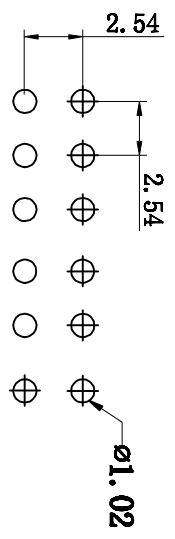
RECOMMENDED PCB LAYOUT COMPONENT SIDE VIEW
