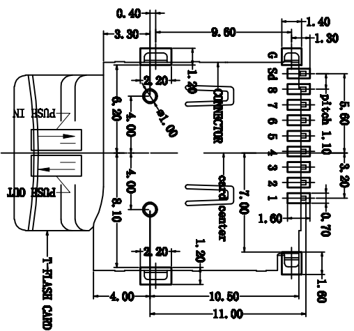
P.C.B. LAYOUT TOLERANCE: ±0.05
