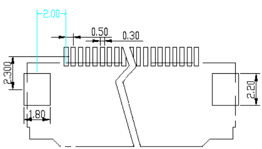
PCB
