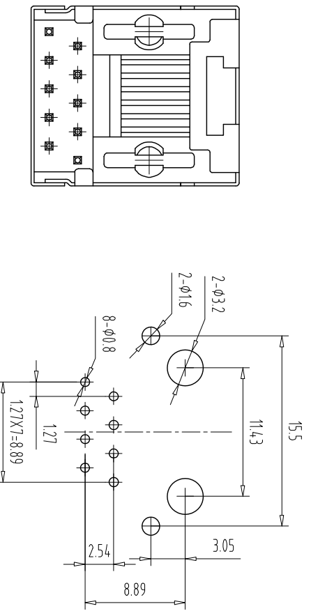
PC Board Layout Component Side Shown
