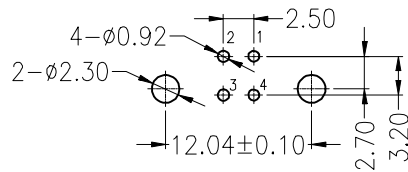
RECOMMENDED P.C.B HOLE LAYOUT TOP VIEW(TOLERANCE:±0.10)
