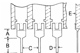
DEVICE FOOTPRINT
