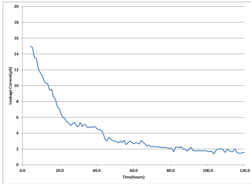
Fig 10: Leakage Current
