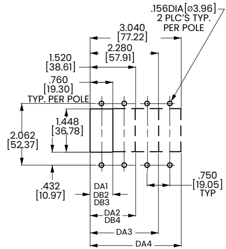
PANEL CUTOUT DETAIL TOLERANCES +.005 [.12]
