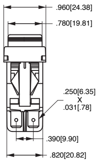
8 TERMINAL BASE W/BARRIERS
