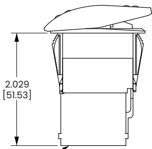
SWITCH SHOWN WITH VCH CONNECTOR 8 TERMINAL
