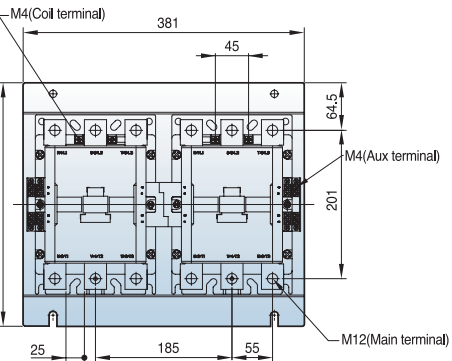
CC265 ~ CC400 reversing combination shown with aux contacts
